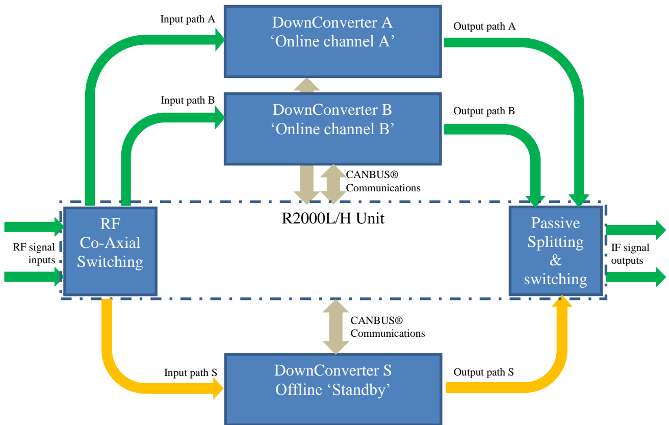
P7xxx series DownConverter in 2+1 redundancy using R2000L/H
